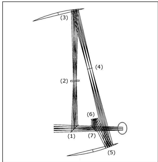
Figure 4. OSCA ray-trace. The sequence of optical components is numbered and the original NAOMI beam (without OSCA) is overlaid to show the focus at INGRID (circled) unchanged.
