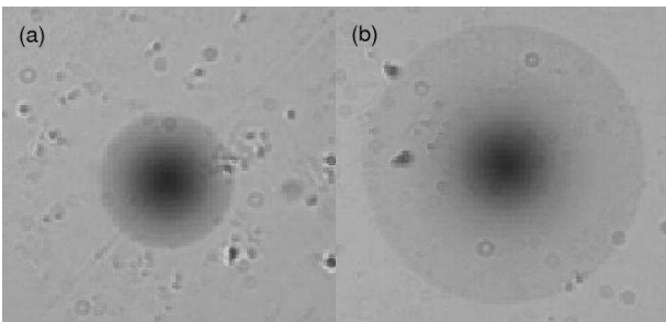
Figure 3. White light images of the OSCA Gaussian profiled HEBS occulting masks. Speckles are dust in the CCD camera.
